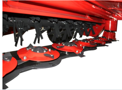
HARMAK BİÇME TABLASI STRONG MOWING UNIT
