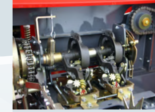
RASSPE BAĞLAMA TİPİ RASSPE THREAD BINDER TYPE
