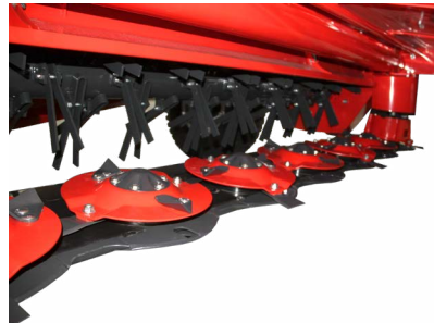
HARMAC BİÇME TABLASI STRONG MOWING UNIT
